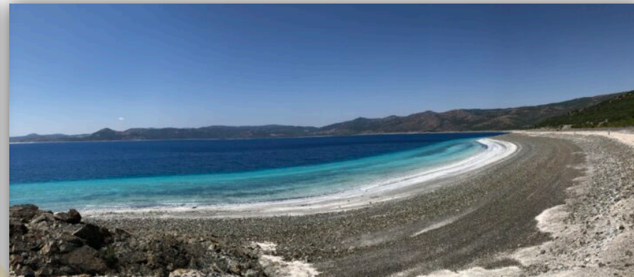
Northeastern shore of Lake Salda Photo credit: Bradley Garczynski
