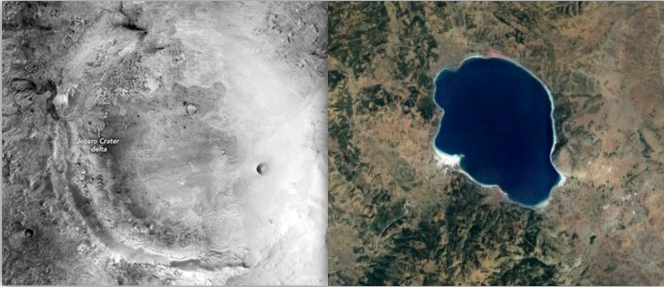
Jezero Crater in Mars (left) and Lake Salda (right) Photo credit: NASA and Google
