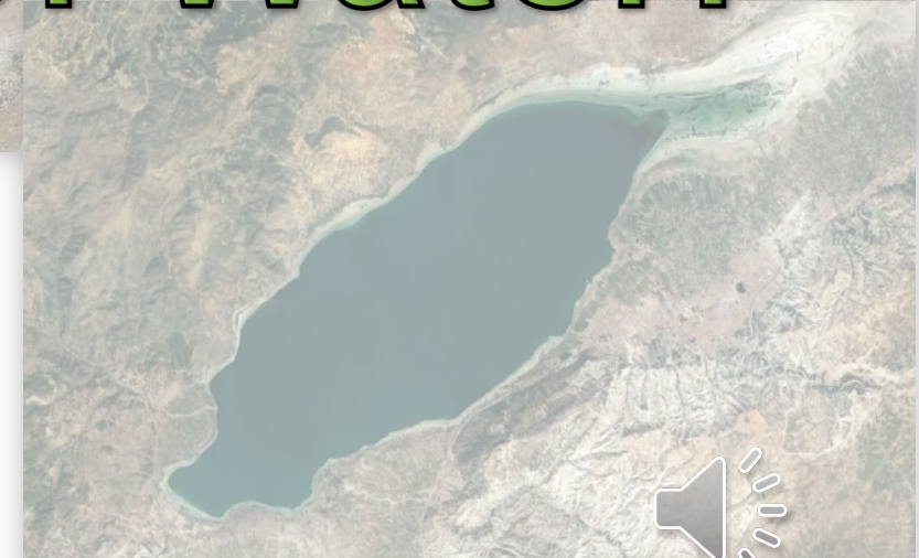
Lake Burdur Photo credit: www.ozelkalem.com.tr and Google
